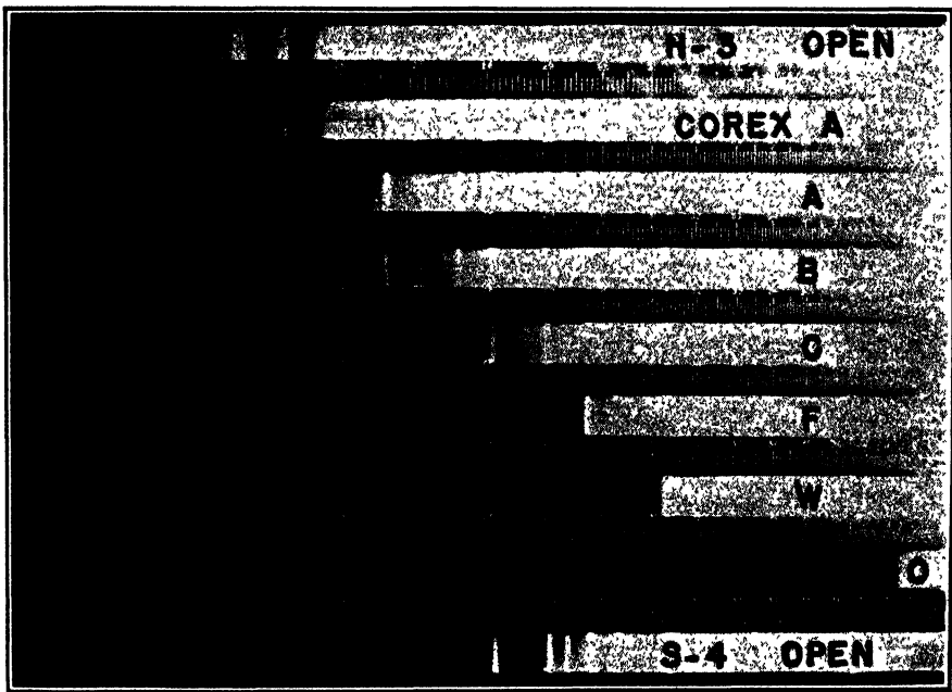
FIGURE 2. Spectrograms of light transmission with type H-3 lamp, open and with filters "Corex A," "A," "B," "C," "F," window glass, and "Noviol O." Bottom spectrogram type S-4 lamp without filter.
