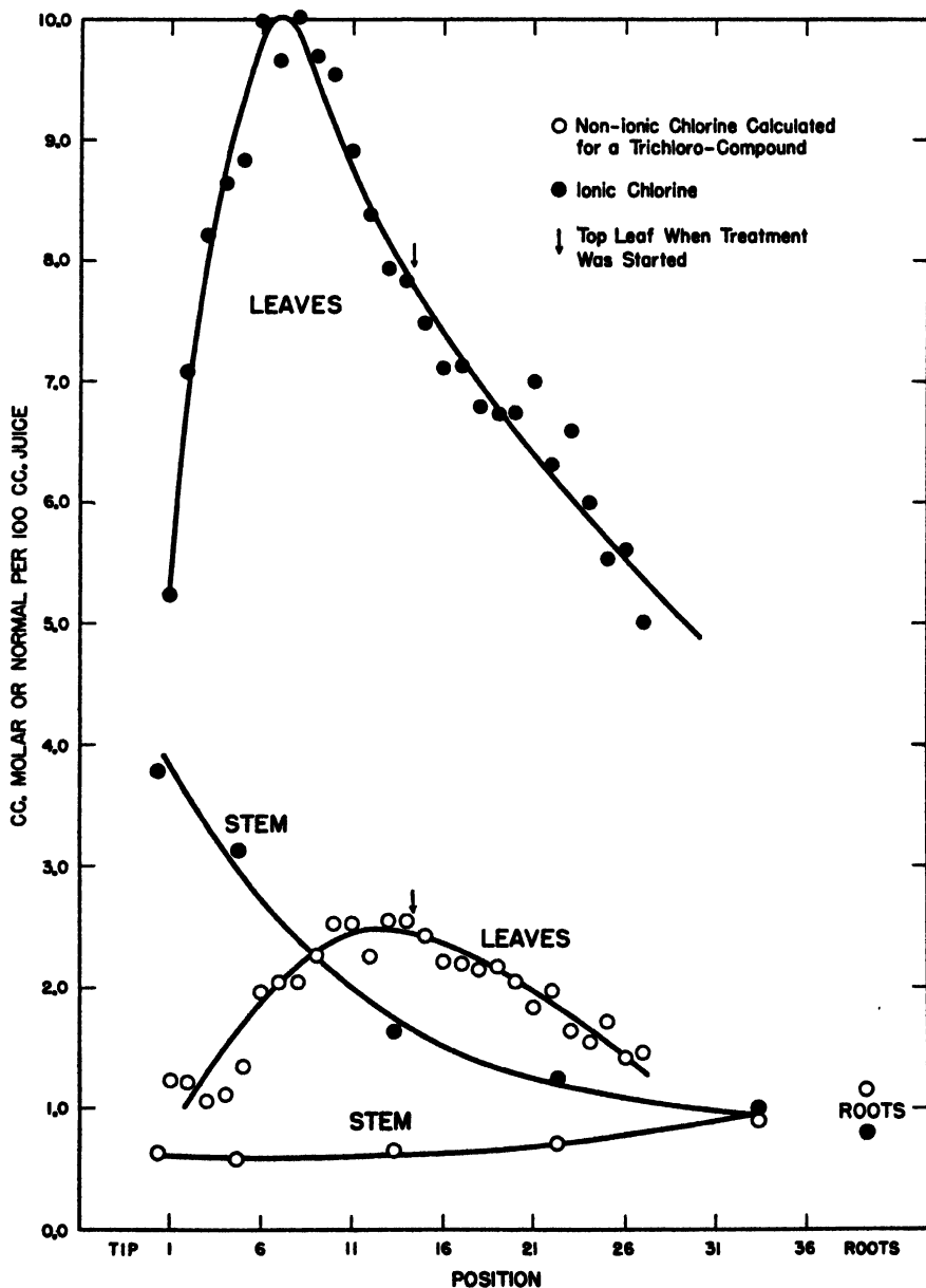
FIGURE 2. Distribution of ionic and non-ionic chlorine in tobacco plants grown with chloral hydrate added to the nutrient medium.
